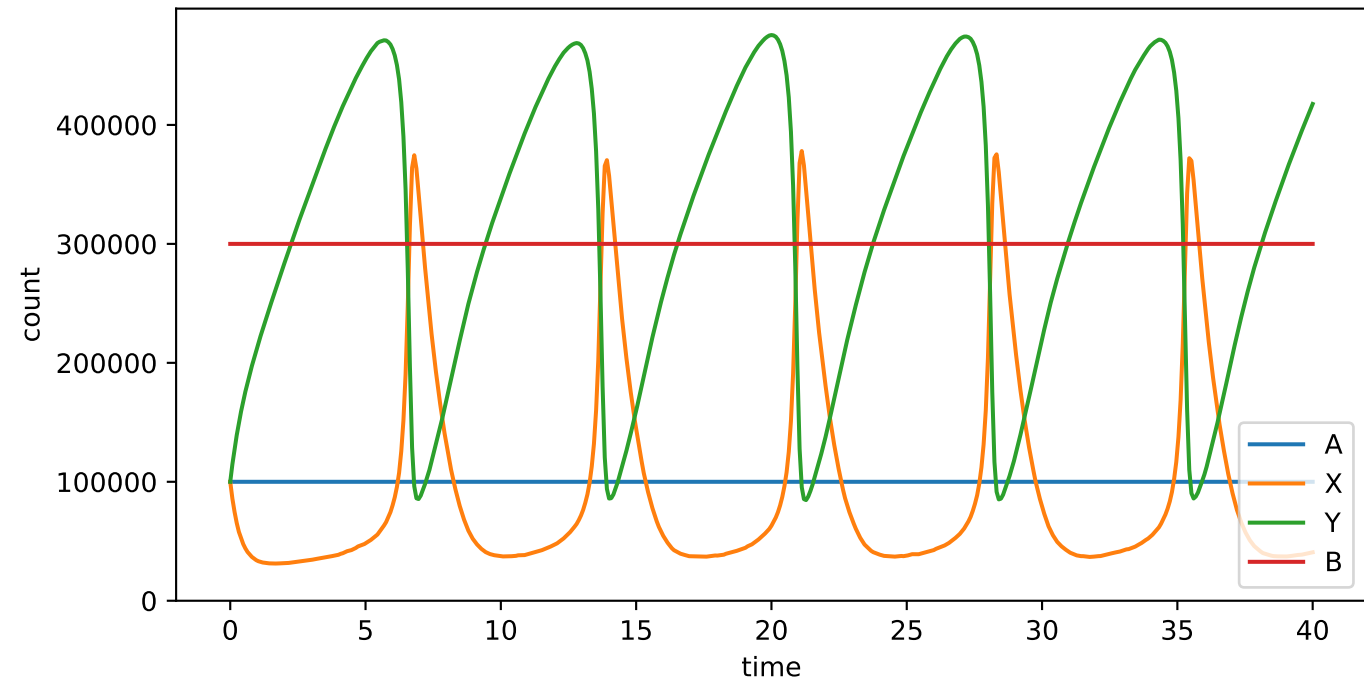
Order-3 Brusselator: rebop, n=10^5
